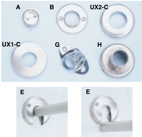
UX1-E 1" o.d. COLLAPSABLE
